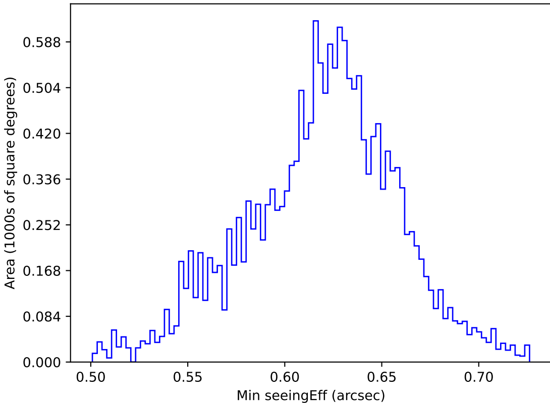
weather_cloudso36v3.4_10yrs WFD r band: Min seeingEff
