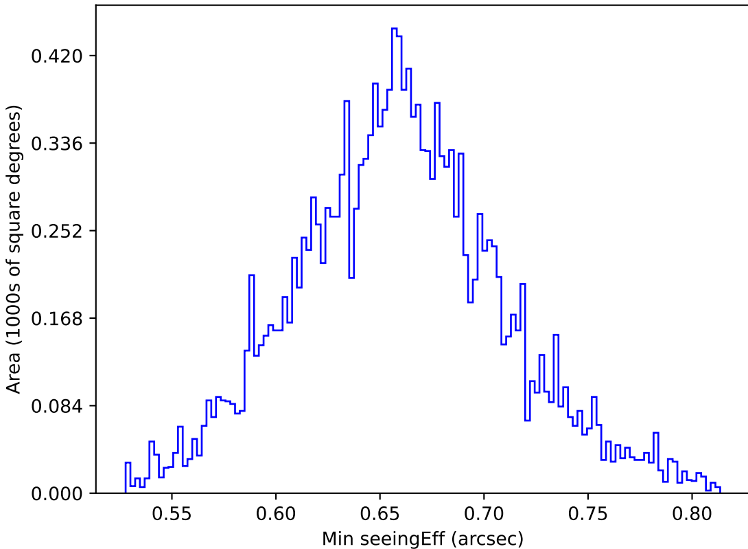
weather_cloudso36v3.4_10yrs WFD g band: Min seeingEff
