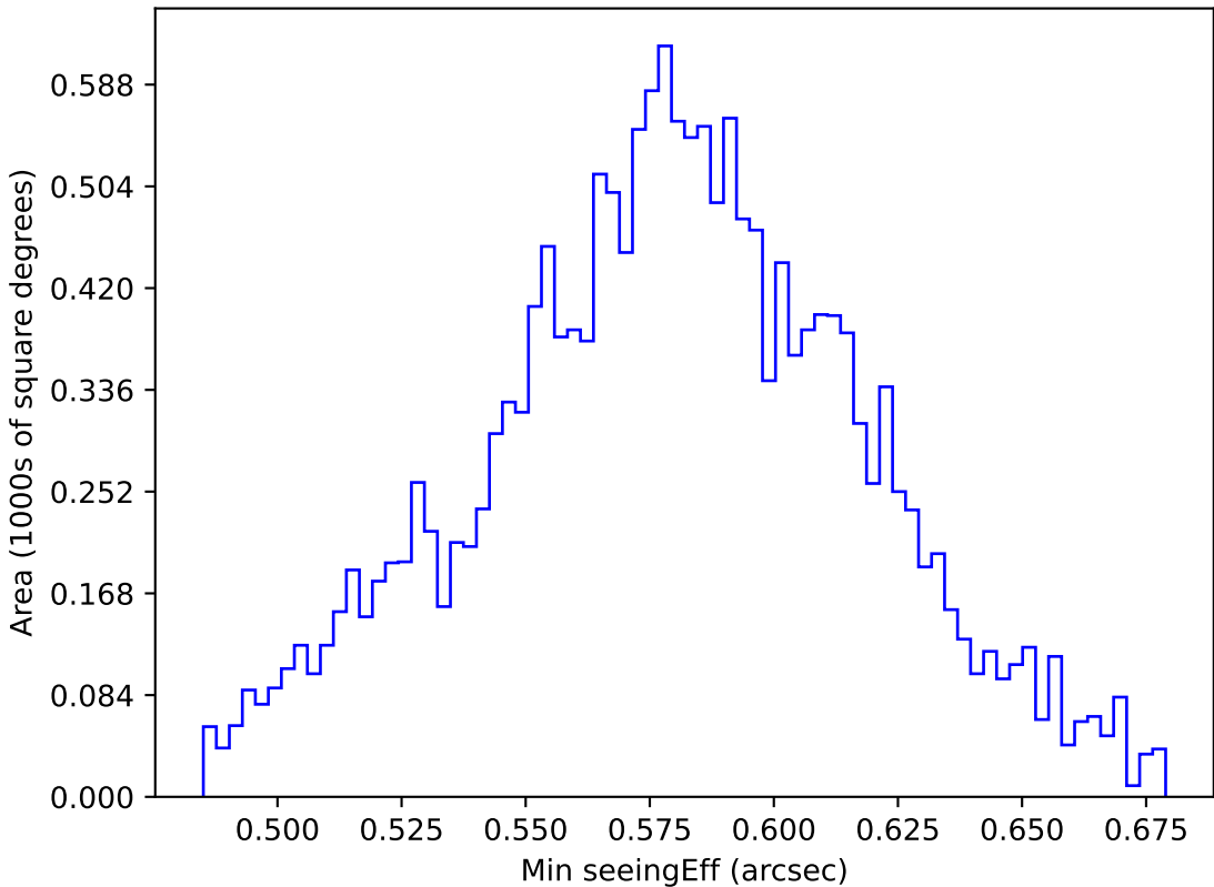
weather_cloudso36v3.4_10yrs WFD all bands: Min seeingEff
