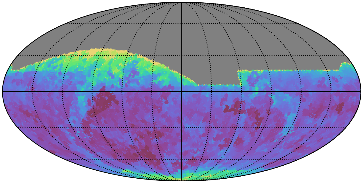
weather_cloudso36v3.4_10yrs All sky z band: Min seeingEff
