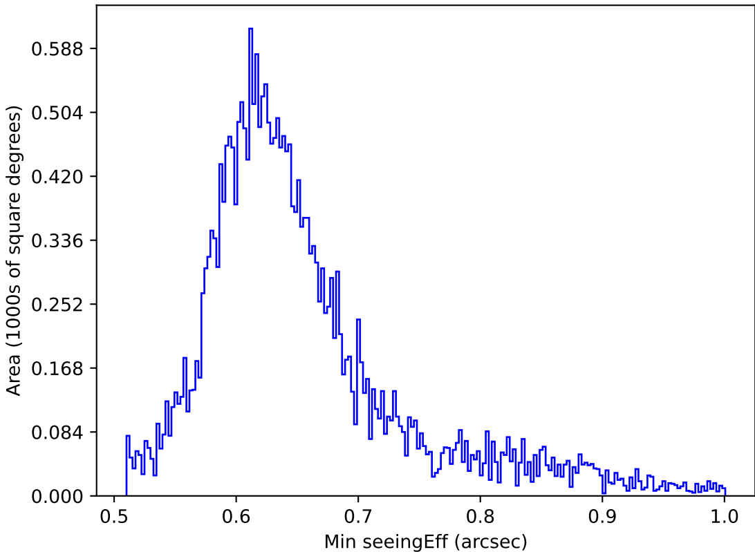
weather_cloudso36v3.4_10yrs All sky z band: Min seeingEff
