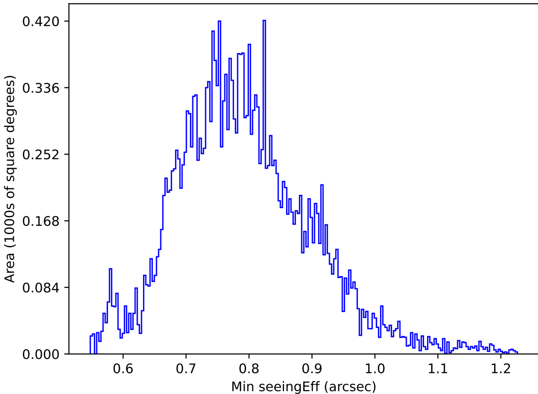
weather_cloudso36v3.4_10yrs All sky u band: Min seeingEff
