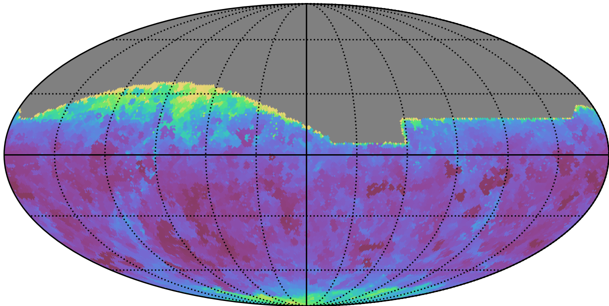
weather_cloudso36v3.4_10yrs All sky i band: Min seeingEff
