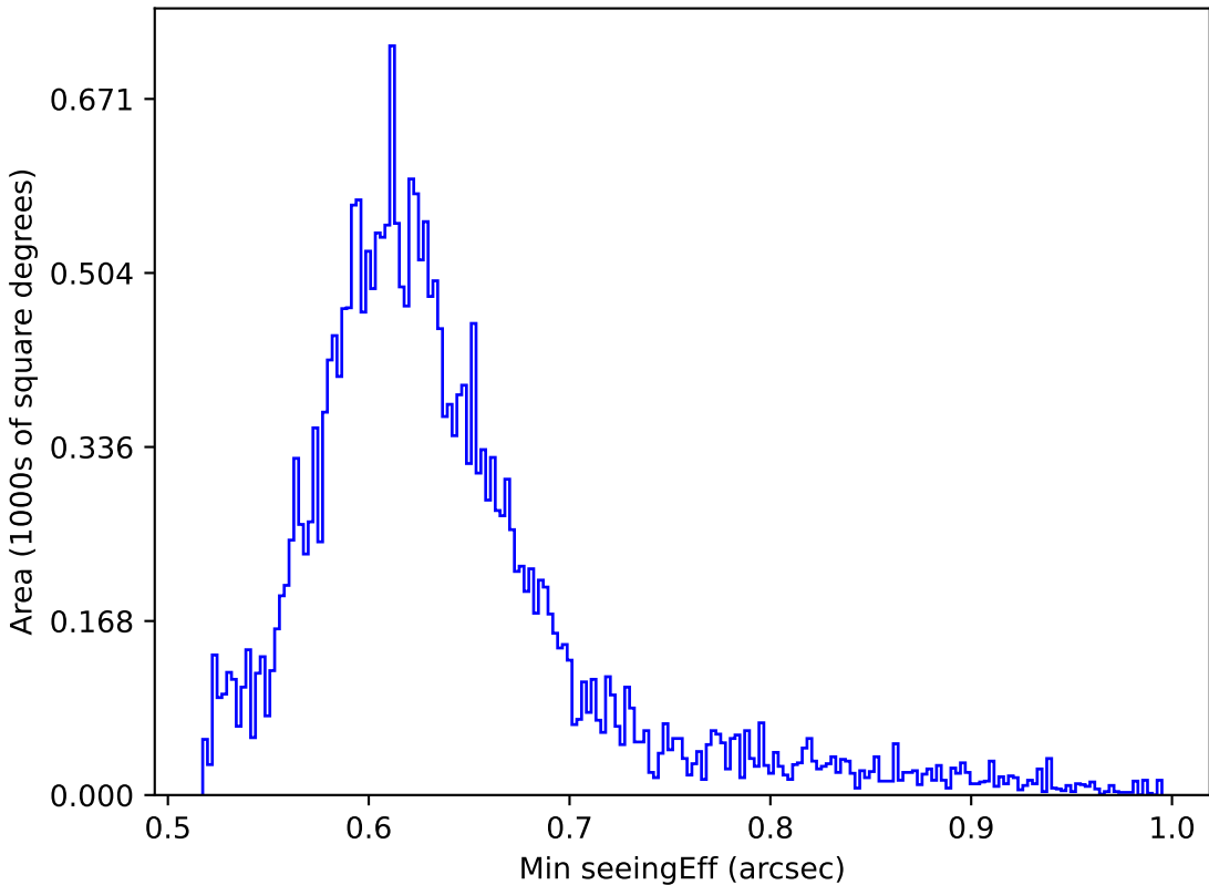
weather_cloudso36v3.4_10yrs All sky i band: Min seeingEff
