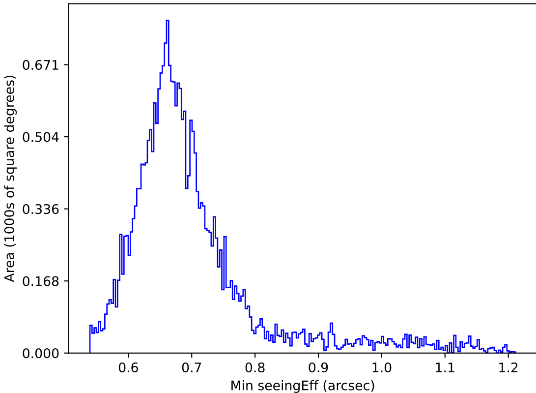
weather_cloudso36v3.4_10yrs All sky g band: Min seeingEff
