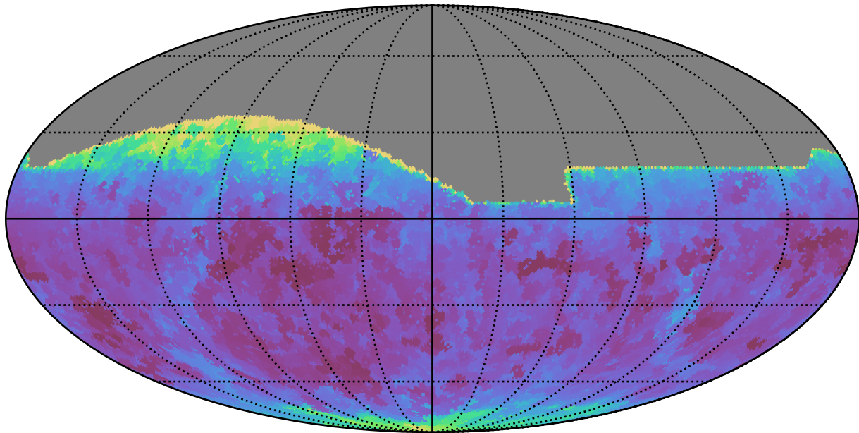
weather_cloudso36v3.4_10yrs All sky all bands: Min seeingEff
