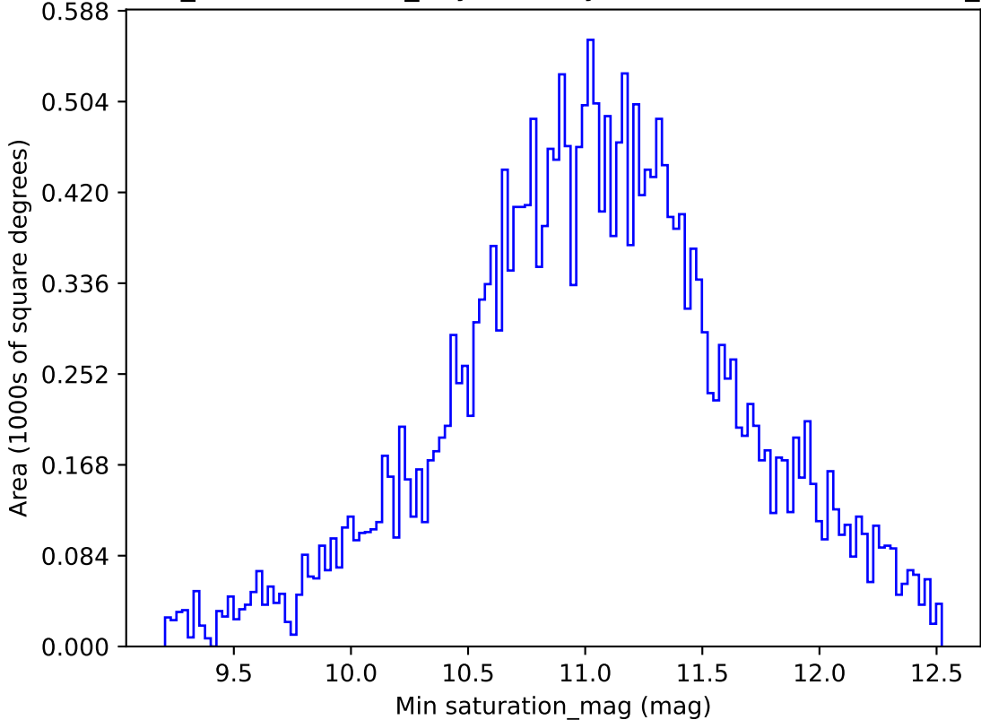
weather_cloudso36v3.4_10yrs All sky all bands: Min saturation_mag
