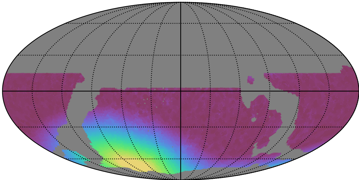
weather_cloudso36v3.4_10yrs WFD z band: Min moonDistance
