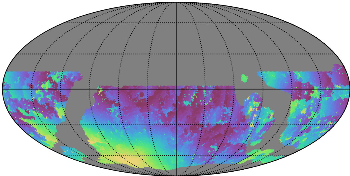
weather_cloudso36v3.4_10yrs WFD u band: Min moonDistance
