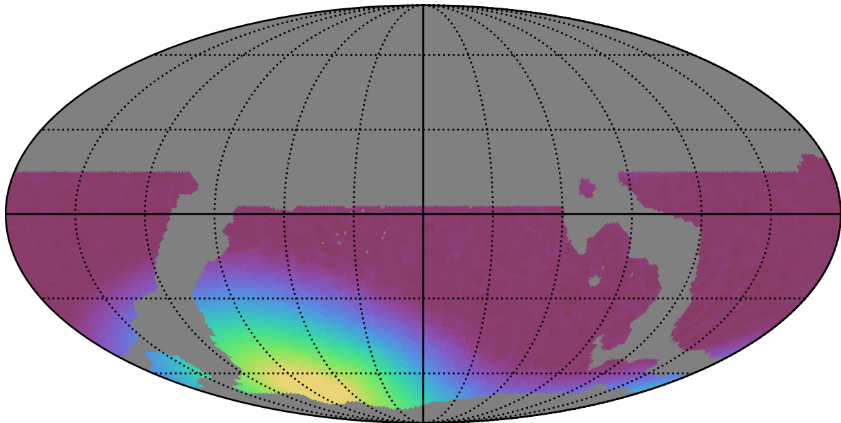
weather_cloudso36v3.4_10yrs WFD all bands: Min moonDistance
