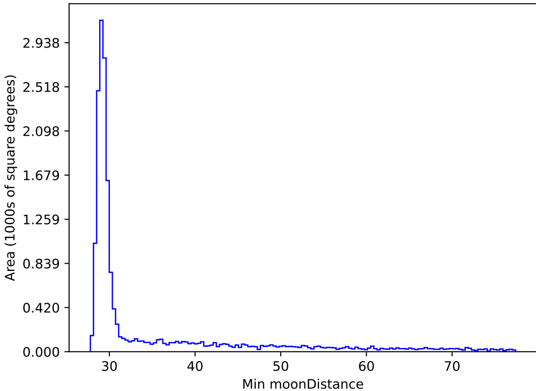
weather_cloudso36v3.4_10yrs WFD all bands: Min moonDistance
