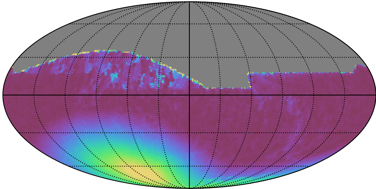
weather_cloudso36v3.4_10yrs All sky z band: Min moonDistance
