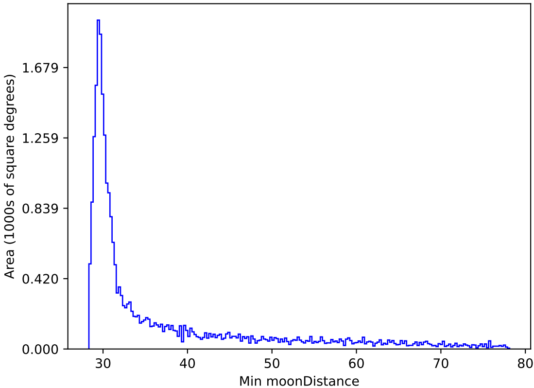
weather_cloudso36v3.4_10yrs All sky z band: Min moonDistance
