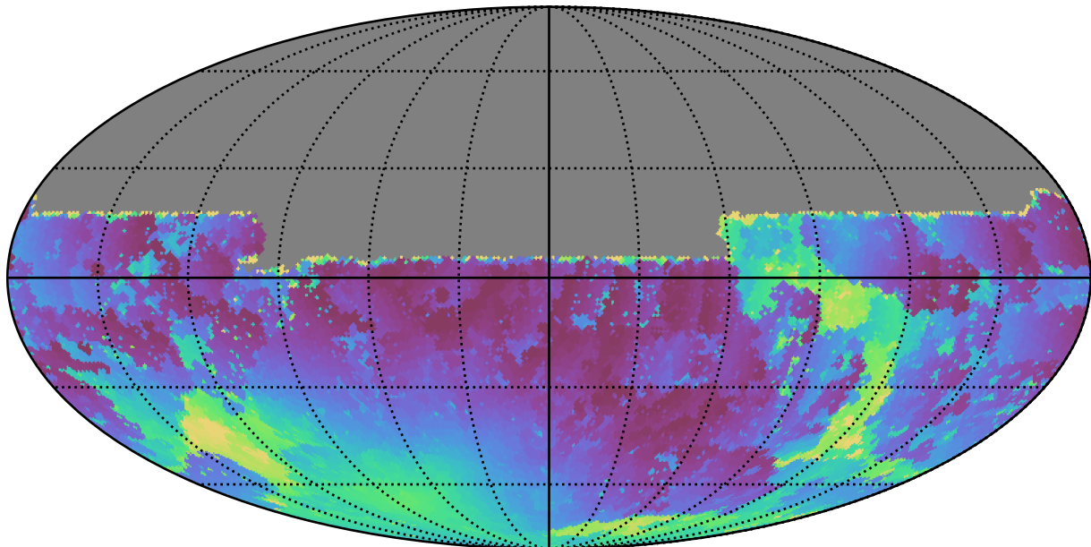
weather_cloudso36v3.4_10yrs All sky u band: Min moonDistance
