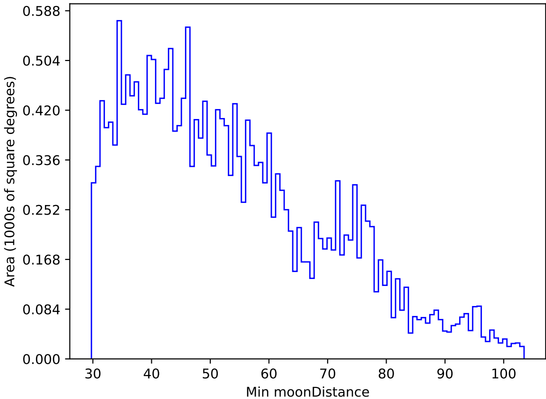
weather_cloudso36v3.4_10yrs All sky u band: Min moonDistance
