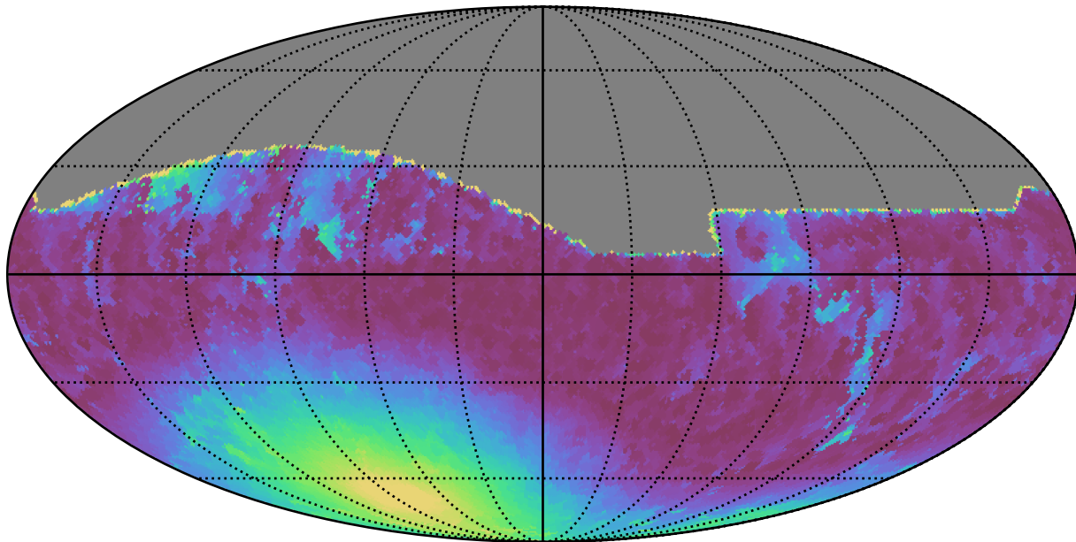
weather_cloudso36v3.4_10yrs All sky r band: Min moonDistance
