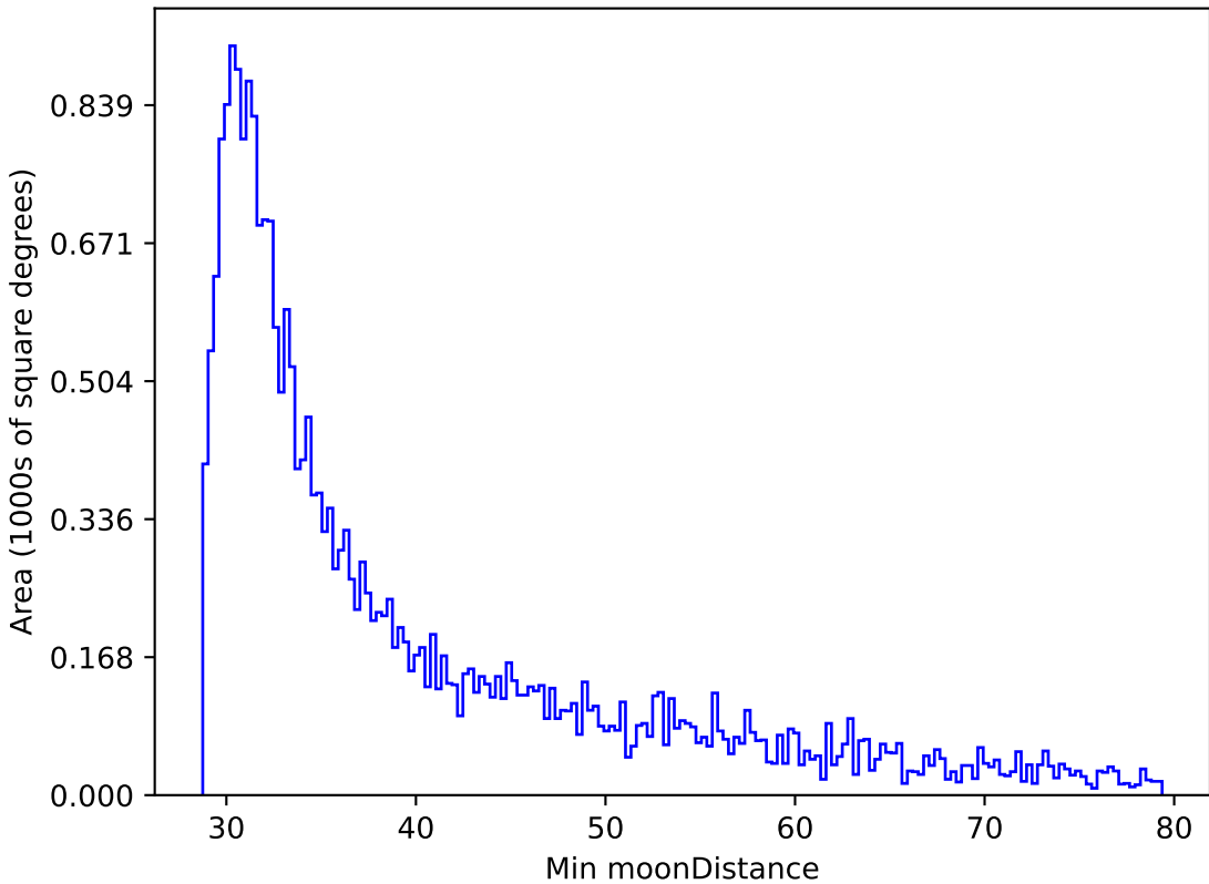
weather_cloudso36v3.4_10yrs All sky r band: Min moonDistance
