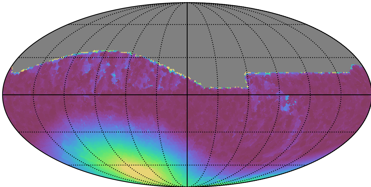
weather_cloudso36v3.4_10yrs All sky i band: Min moonDistance
