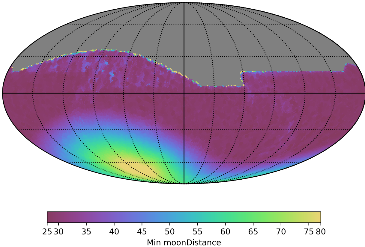
weather_cloudso36v3.4_10yrs All sky all bands: Min moonDistance
