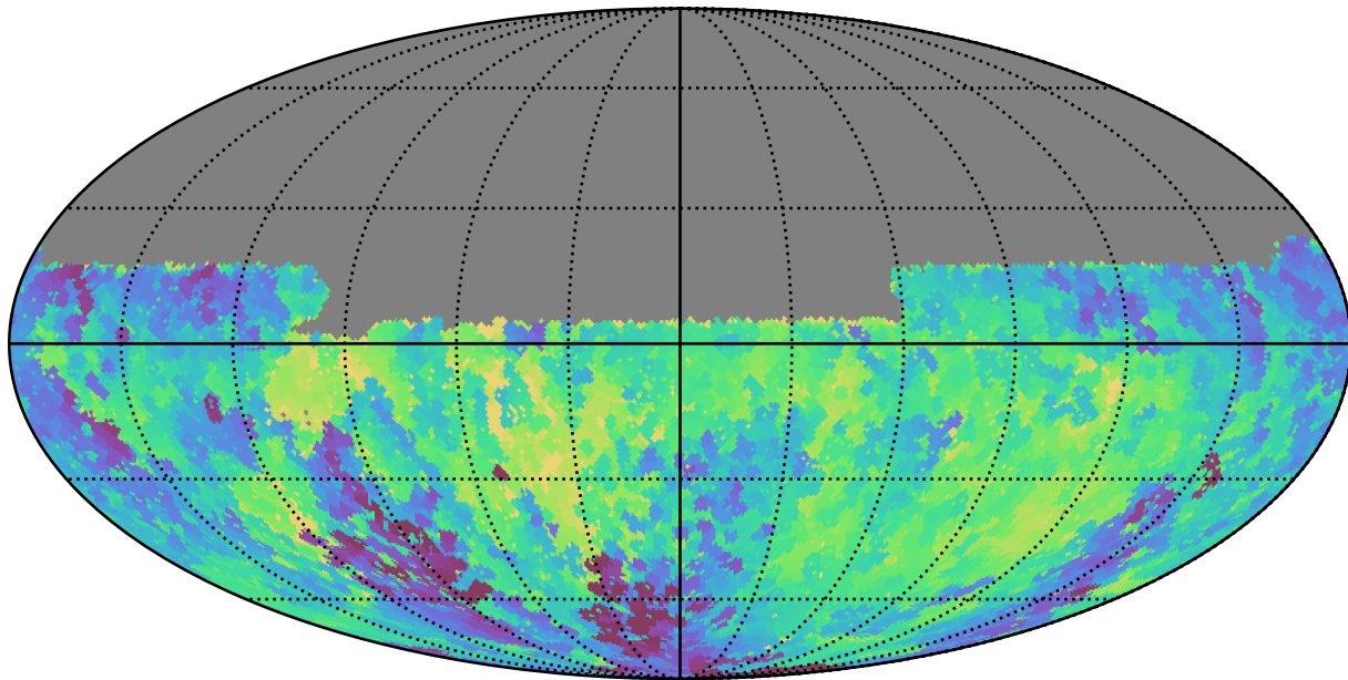
weather_cloudso36v3.4_10yrs Yr 1 y band: Min fiveSigmaDepth
