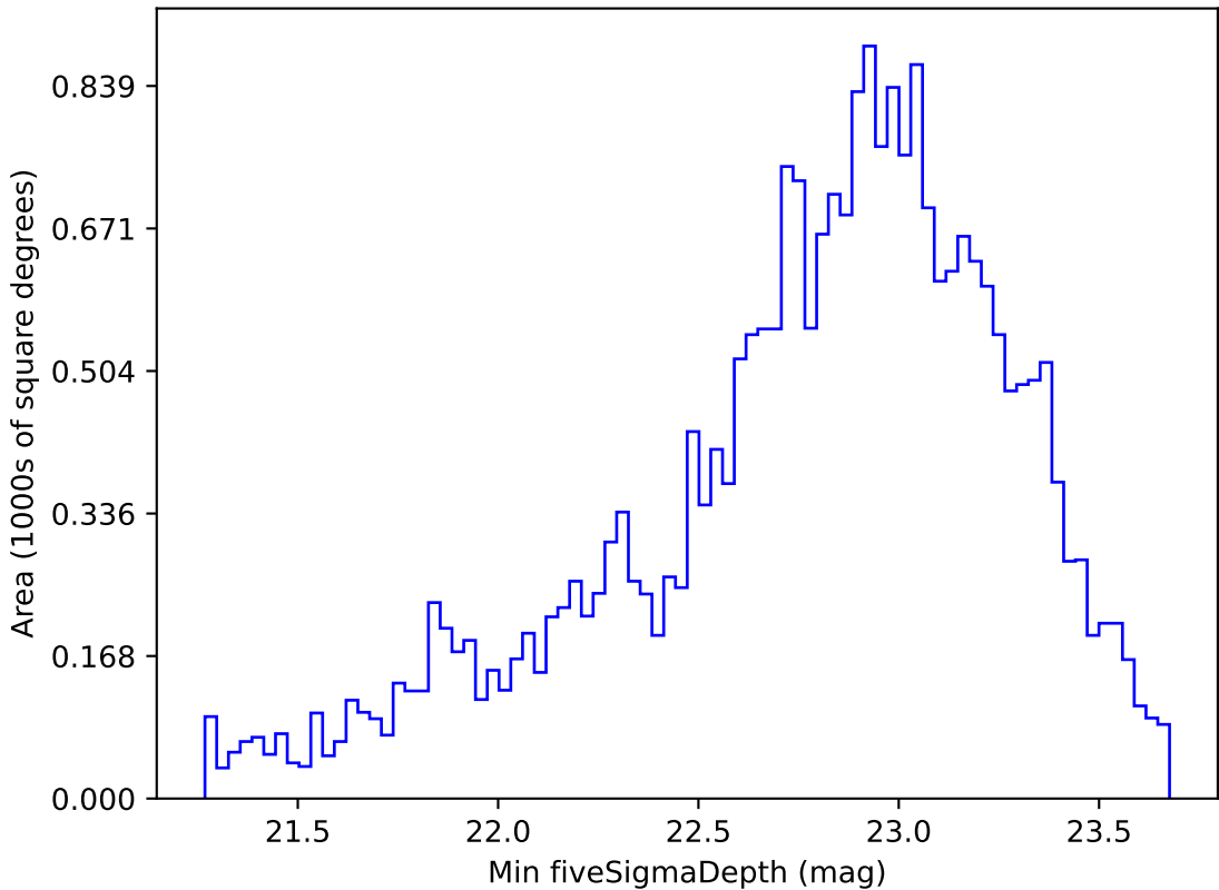
weather_cloudso36v3.4_10yrs Yr 1 i band: Min fiveSigmaDepth
