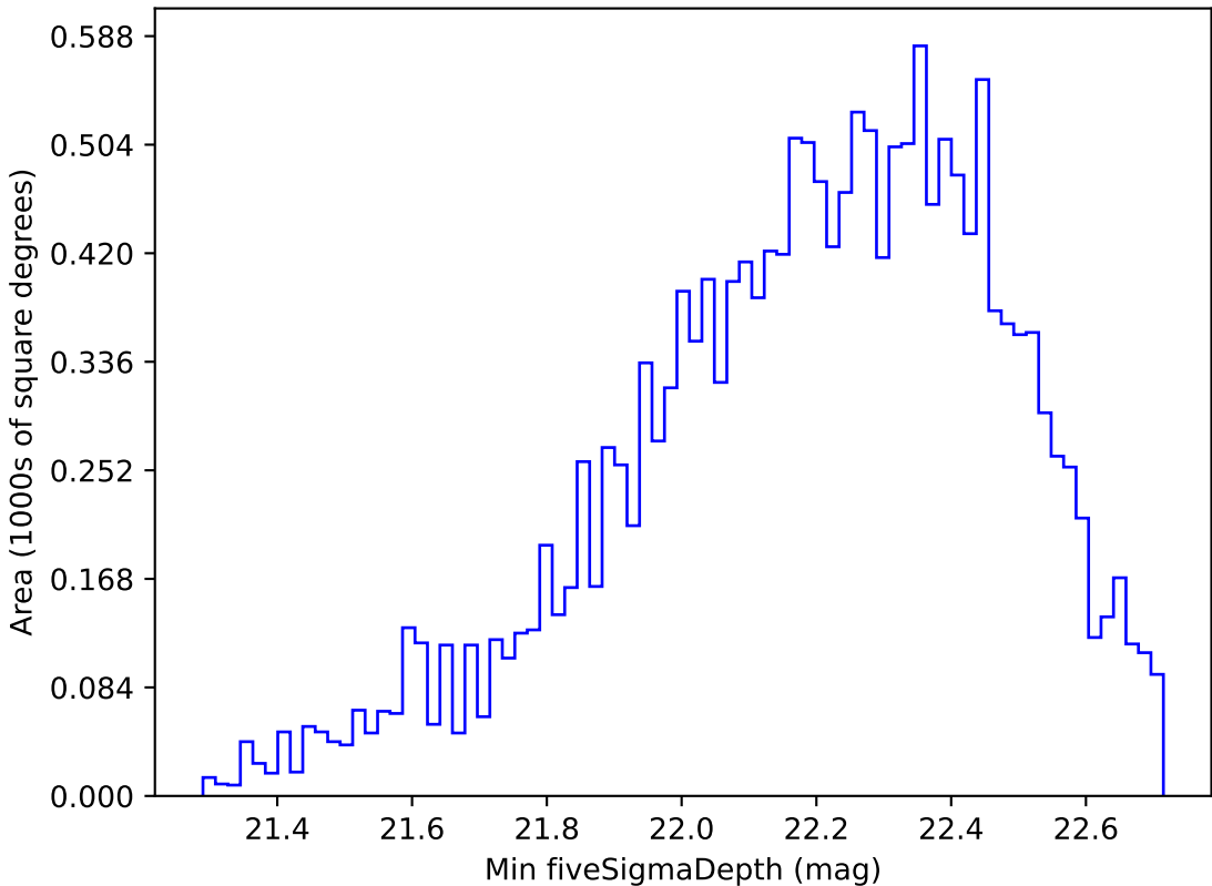
weather_cloudso36v3.4_10yrs WFD u band: Min fiveSigmaDepth
