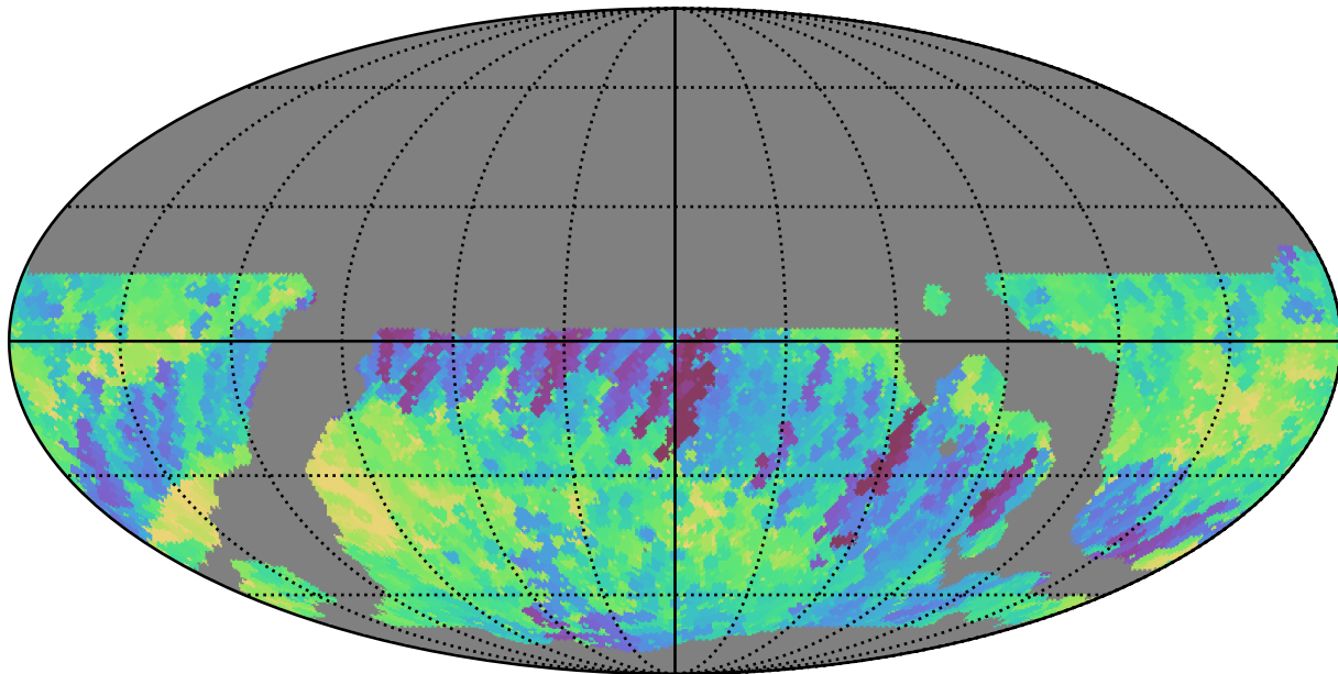
weather_cloudso36v3.4_10yrs WFD r band: Min fiveSigmaDepth
