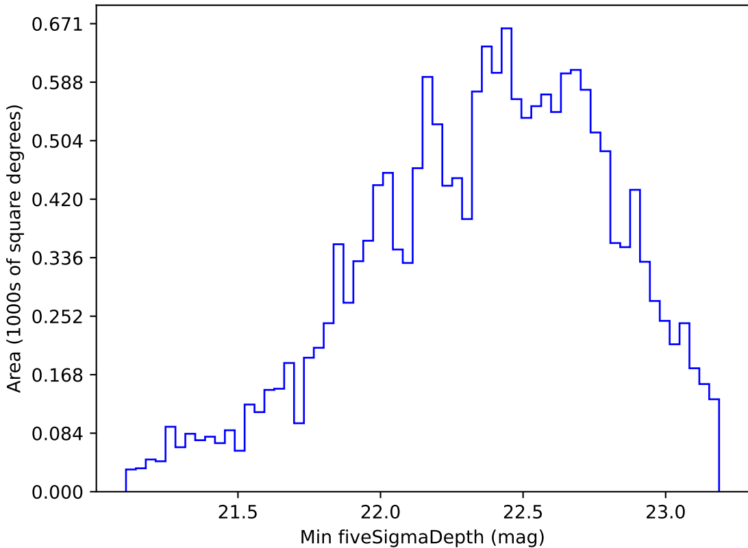
weather_cloudso36v3.4_10yrs WFD r band: Min fiveSigmaDepth
