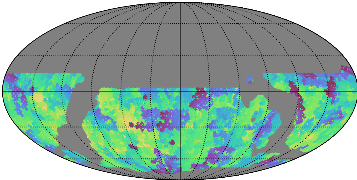
weather_cloudso36v3.4_10yrs WFD g band: Min fiveSigmaDepth
