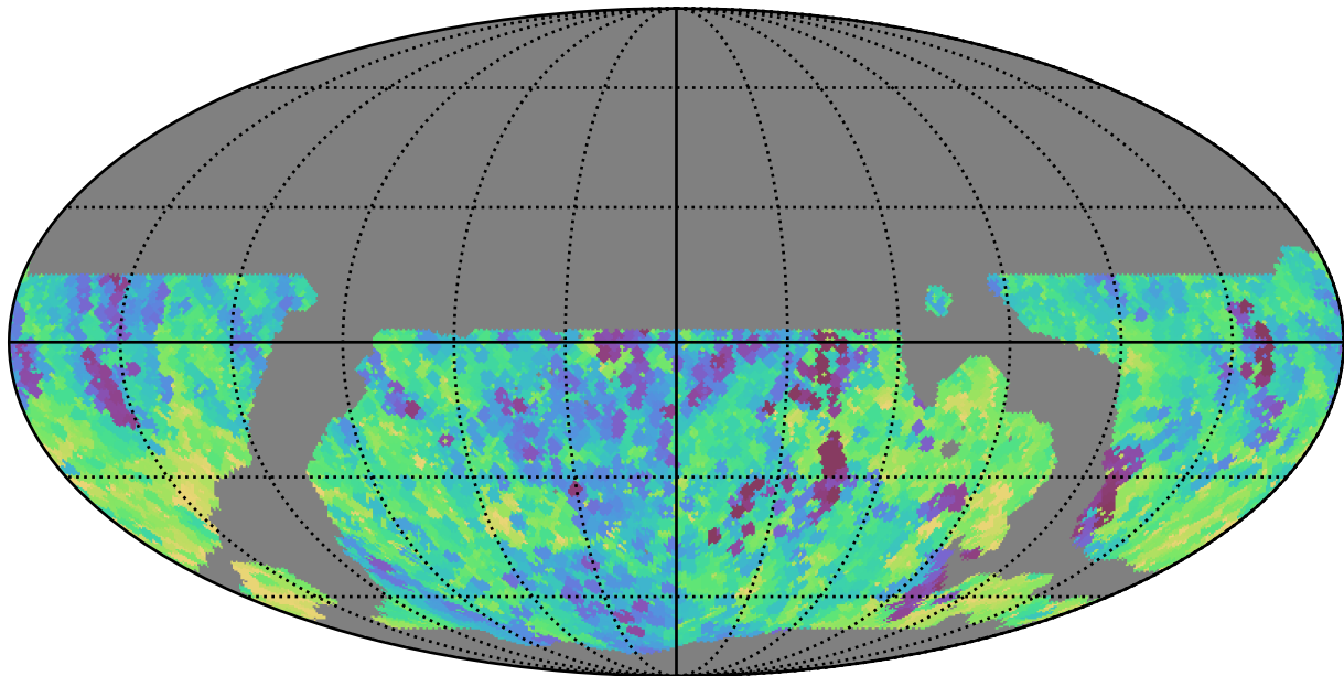
weather_cloudso36v3.4_10yrs WFD all bands: Min fiveSigmaDepth
