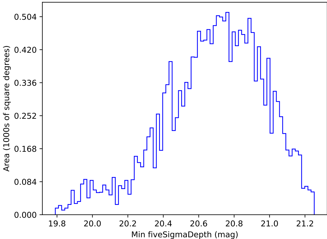
weather_cloudso36v3.4_10yrs WFD all bands: Min fiveSigmaDepth
