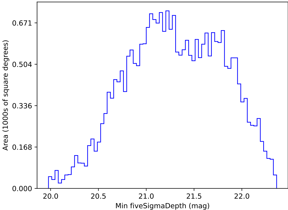
weather_cloudso36v3.4_10yrs All sky z band: Min fiveSigmaDepth
