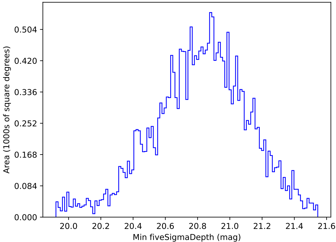
weather_cloudso36v3.4_10yrs All sky y band: Min fiveSigmaDepth
