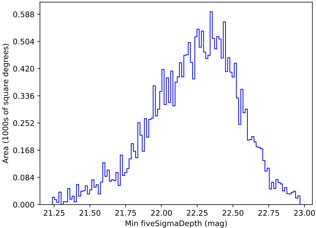
weather_cloudso36v3.4_10yrs All sky u band: Min fiveSigmaDepth
