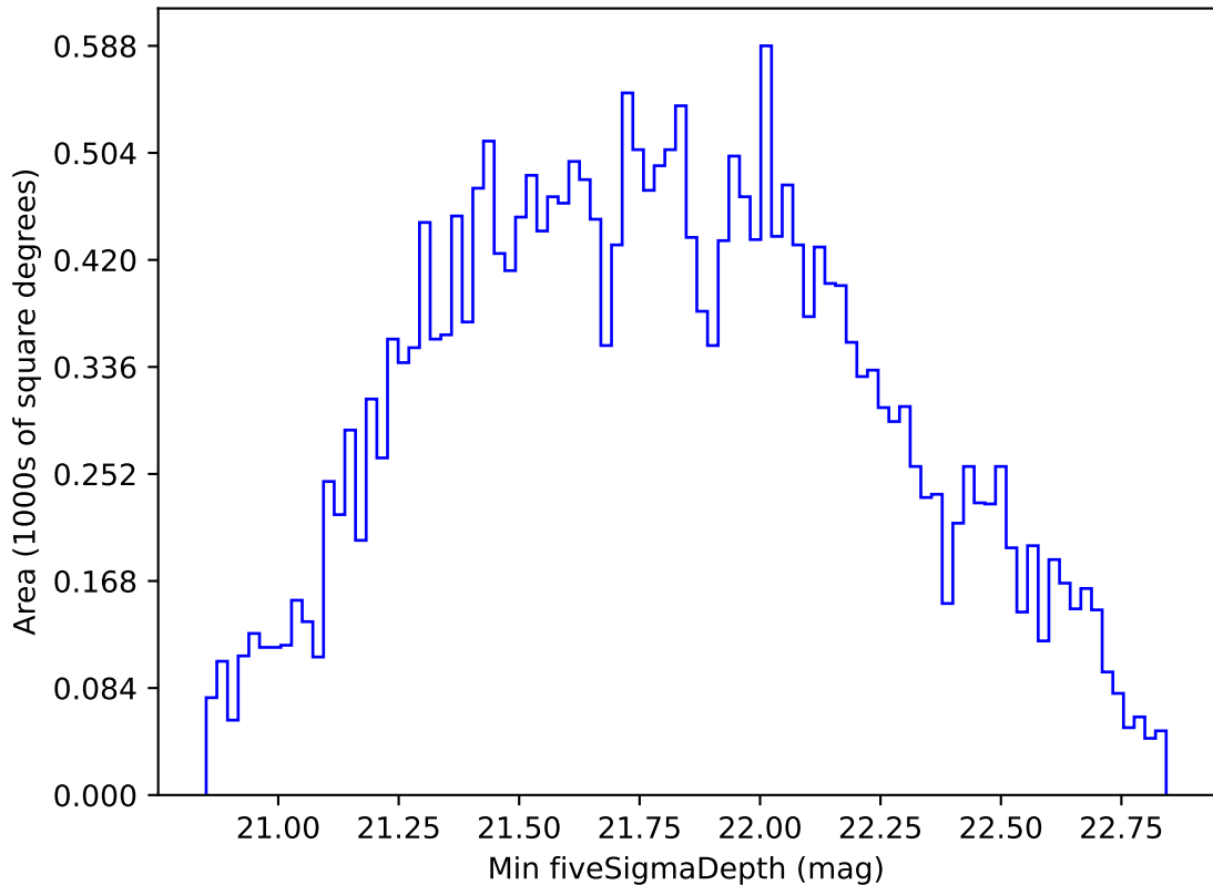
weather_cloudso36v3.4_10yrs All sky i band: Min fiveSigmaDepth
