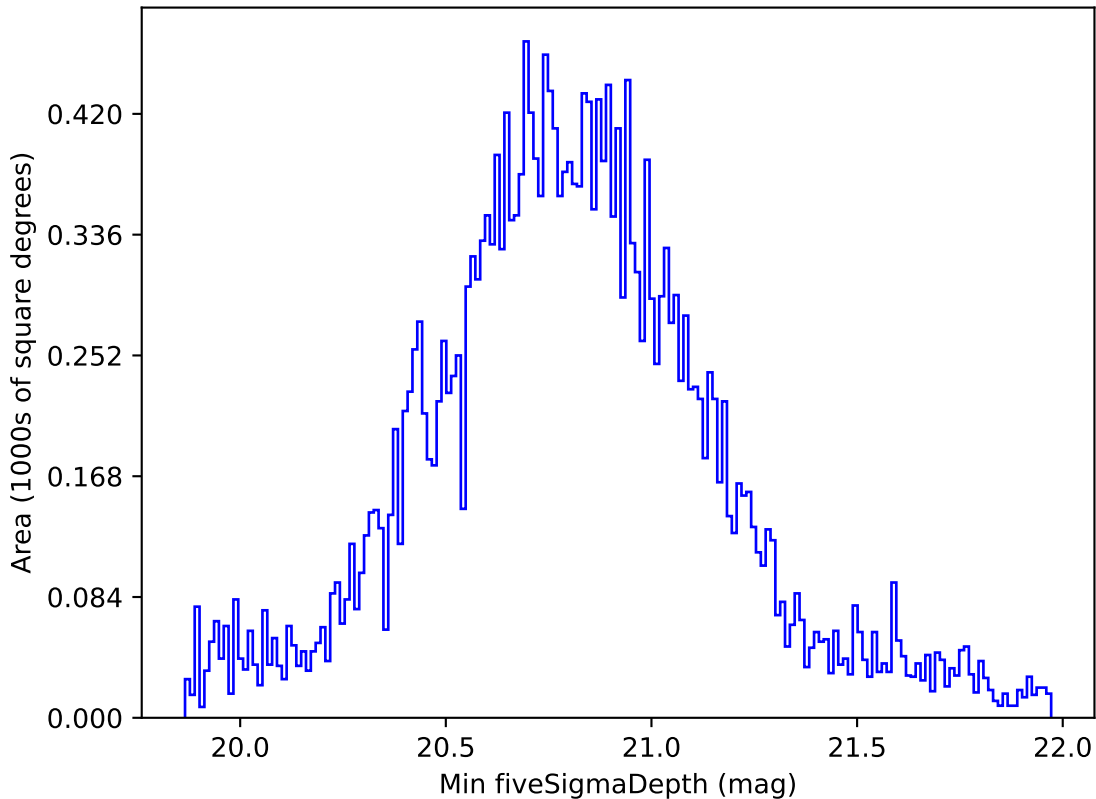
weather_cloudso36v3.4_10yrs All sky all bands: Min fiveSigmaDepth
