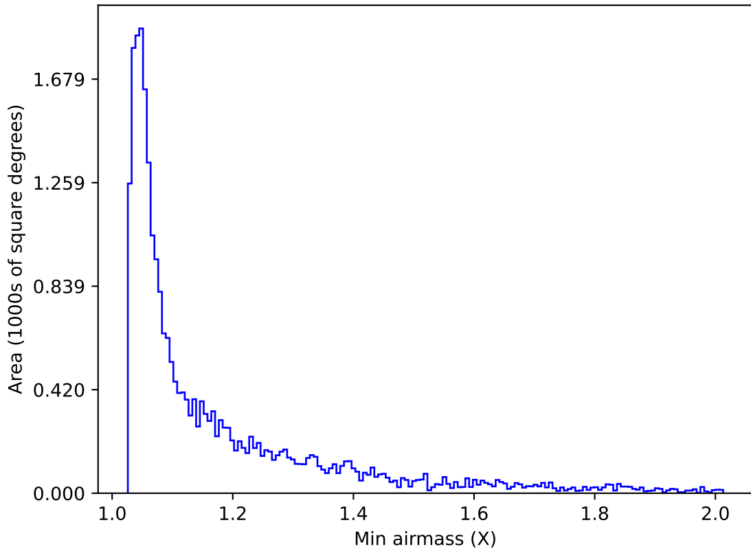
weather_cloudso36v3.4_10yrs Yr 1 z band: Min airmass
