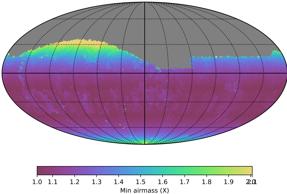
weather_cloudso36v3.4_10yrs Yr 1 g band: Min airmass
