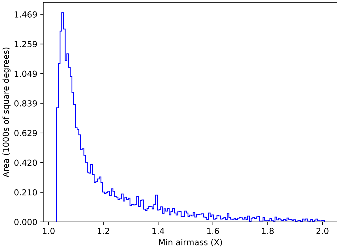
weather_cloudso36v3.4_10yrs Yr 1 g band: Min airmass
