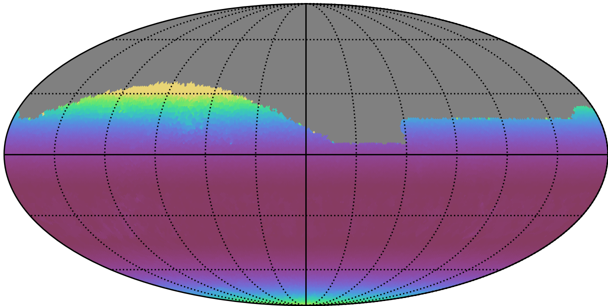
weather_cloudso36v3.4_10yrs Yr 1 all bands: Min airmass
