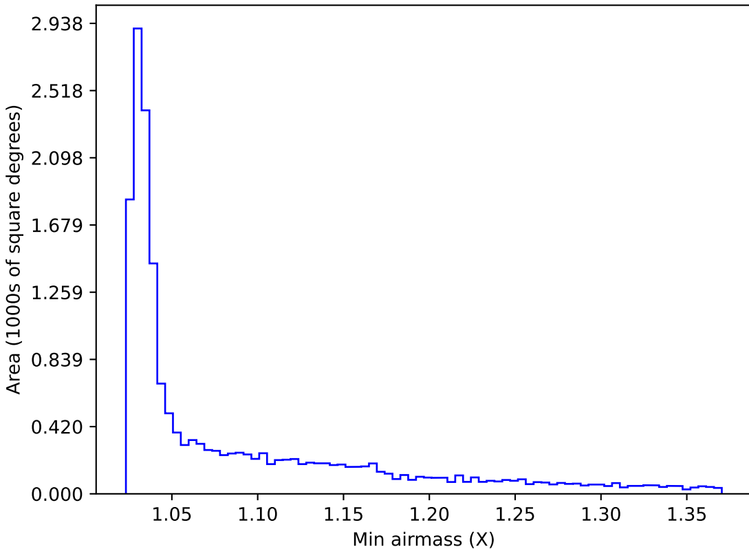
weather_cloudso36v3.4_10yrs WFD y band: Min airmass
