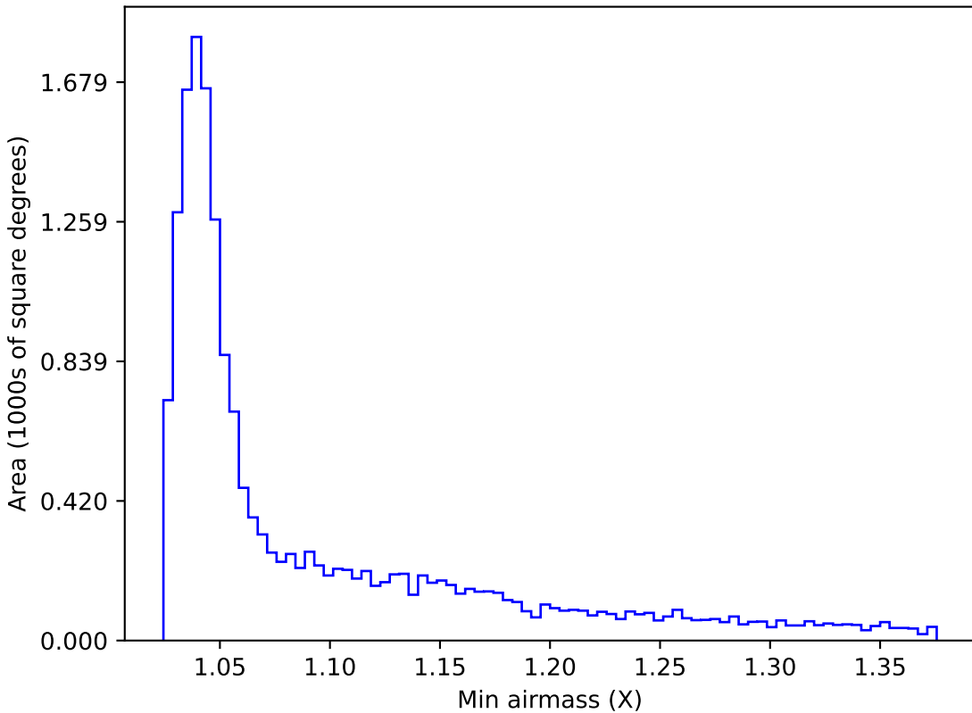
weather_cloudso36v3.4_10yrs WFD u band: Min airmass
