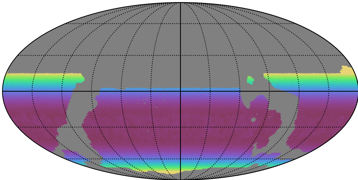
weather_cloudso36v3.4_10yrs WFD r band: Min airmass
