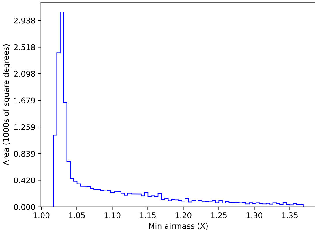
weather_cloudso36v3.4_10yrs WFD r band: Min airmass
