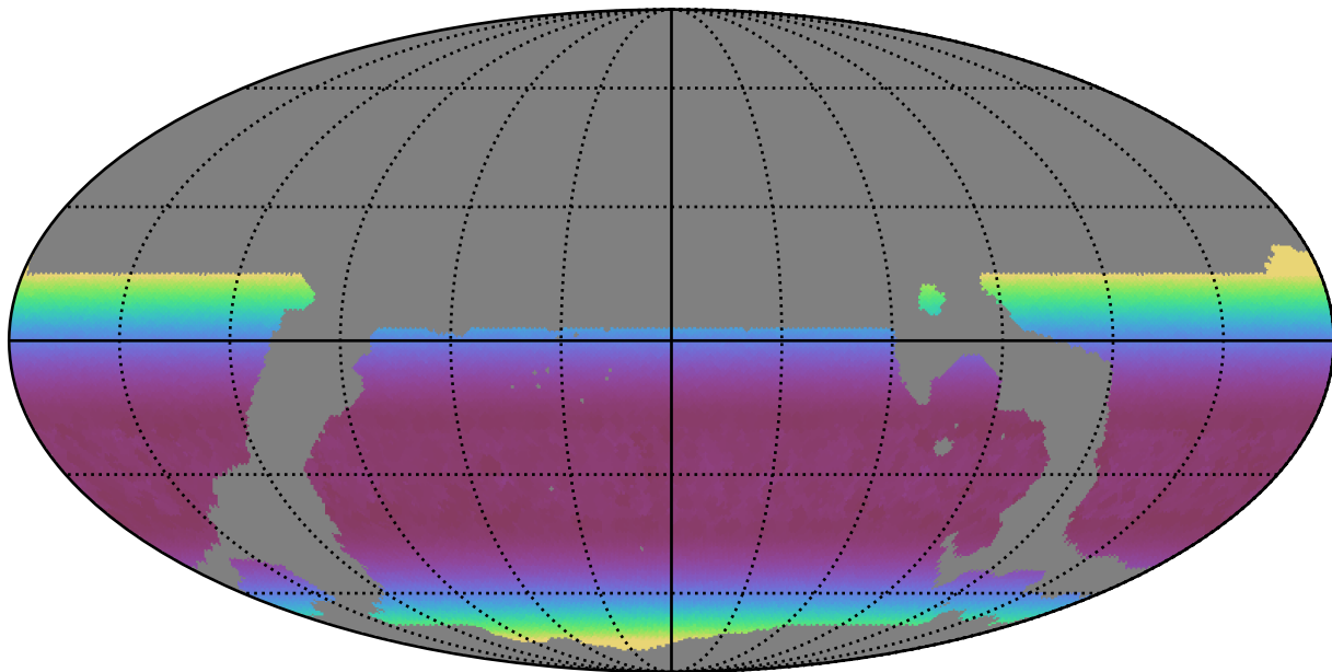
weather_cloudso36v3.4_10yrs WFD i band: Min airmass
