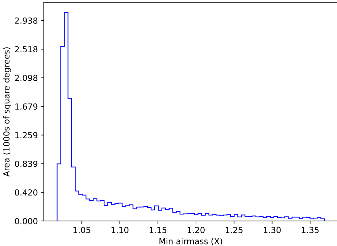
weather_cloudso36v3.4_10yrs WFD i band: Min airmass
