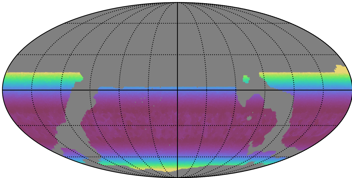
weather_cloudso36v3.4_10yrs WFD g band: Min airmass
