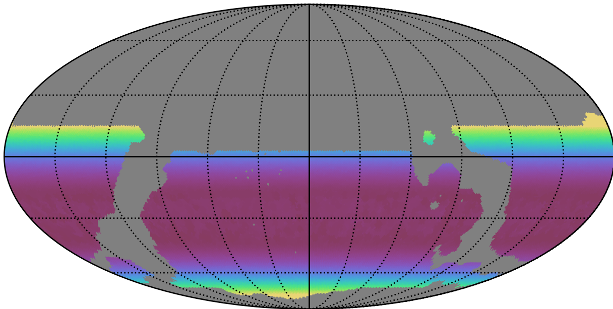
weather_cloudso36v3.4_10yrs WFD all bands: Min airmass
