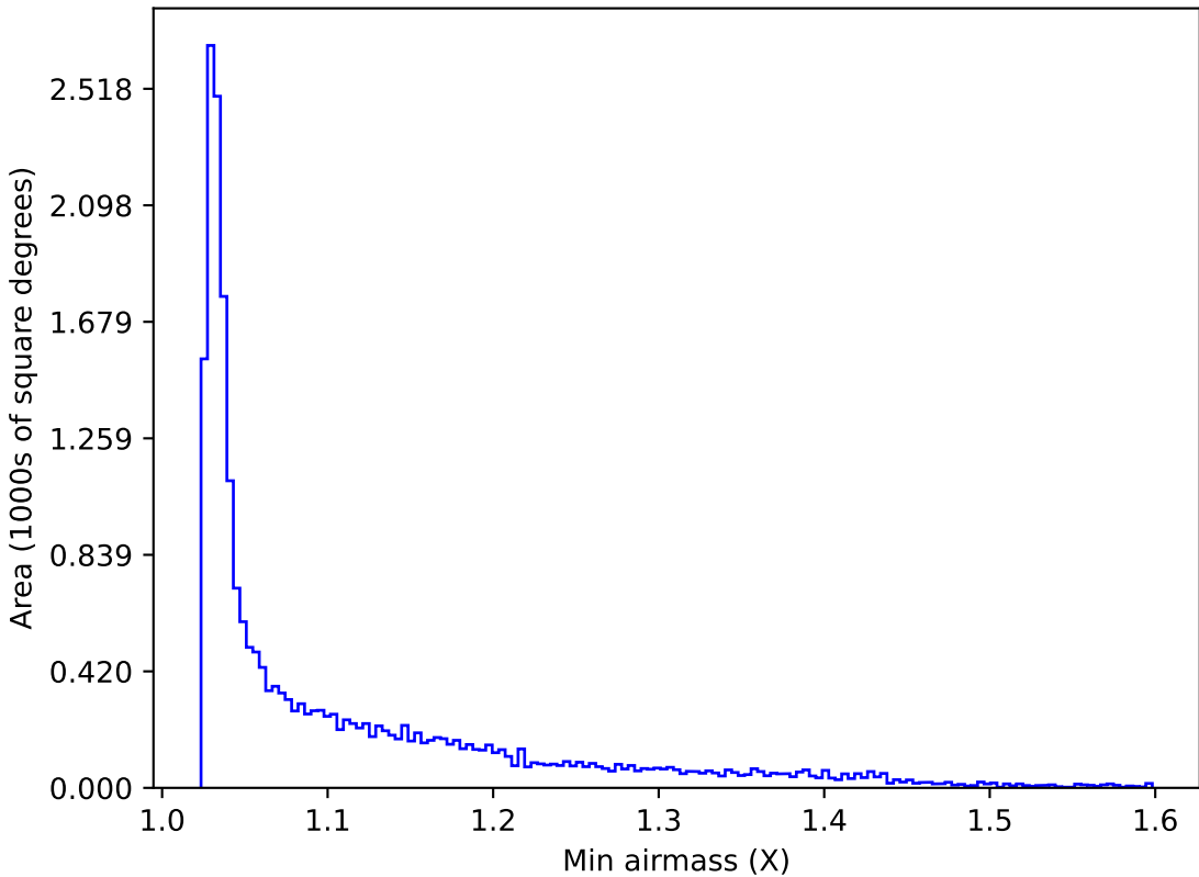
weather_cloudso36v3.4_10yrs All sky y band: Min airmass
