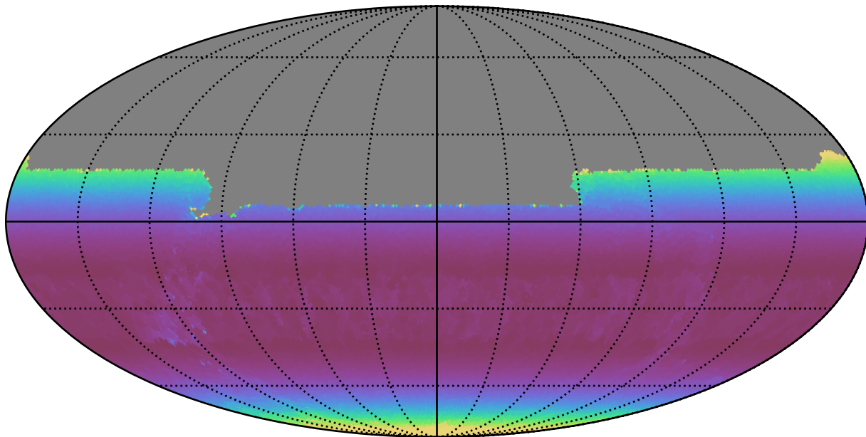
weather_cloudso36v3.4_10yrs All sky u band: Min airmass
